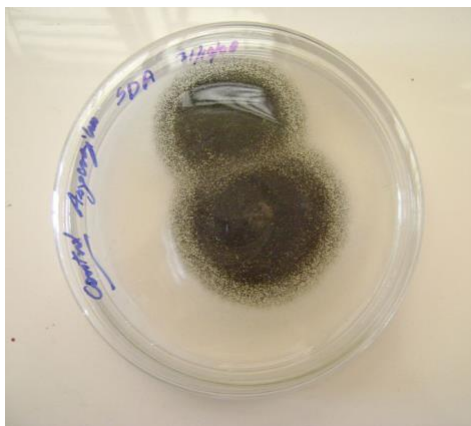
Figure 6: Aspergillus niger mycelium (left); microscopic conidiophore.
